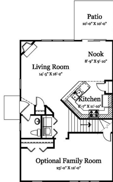
First Floor Plan w/ Opt. Family Room
