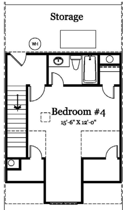
Optional Attic Plan w/ Bedroom & Bath
